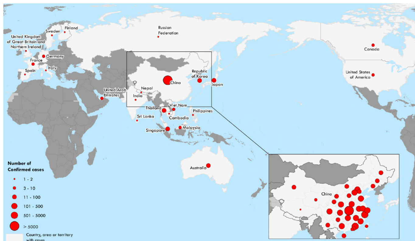
Figure 2 Distribution of 2019-nCoV cases as of 01 February 2020
